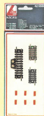
420586 1 piece 1/2 straight track with power connecting terminal 420564R, 2 pieces 1/4 straight track 420563, Insulated fish plates 420017.
